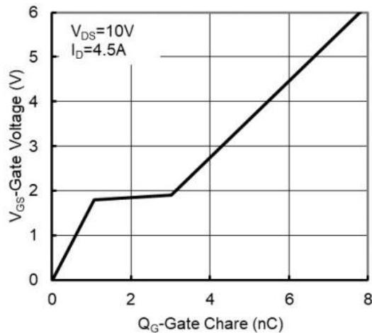
Figure 6: Gate-Charge Characteristics
