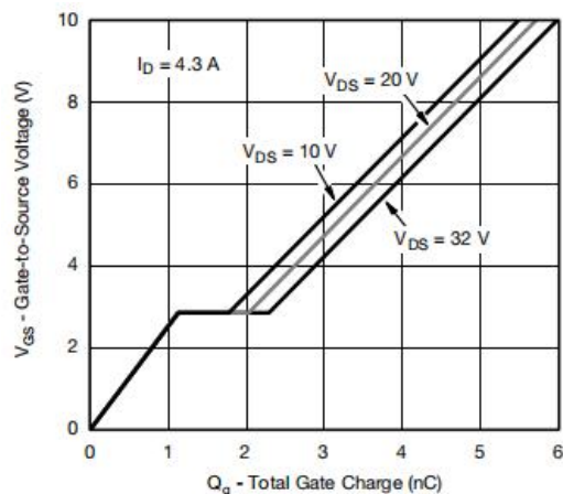
Figure 6: Gate-Charge Characteristics
