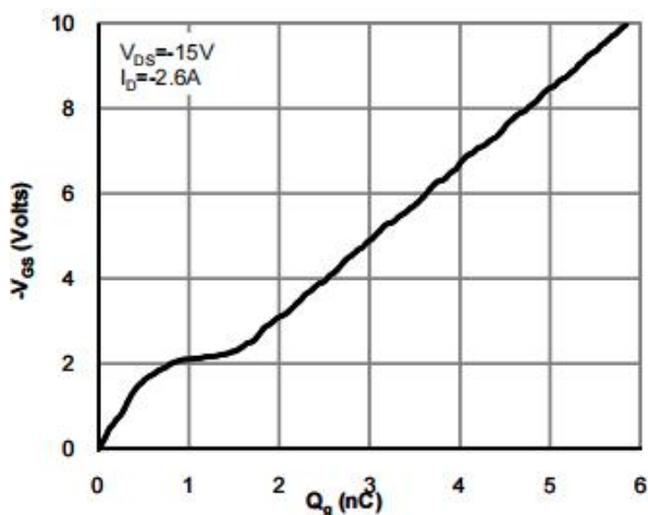
Figure 6: Gate-Charge Characteristics
