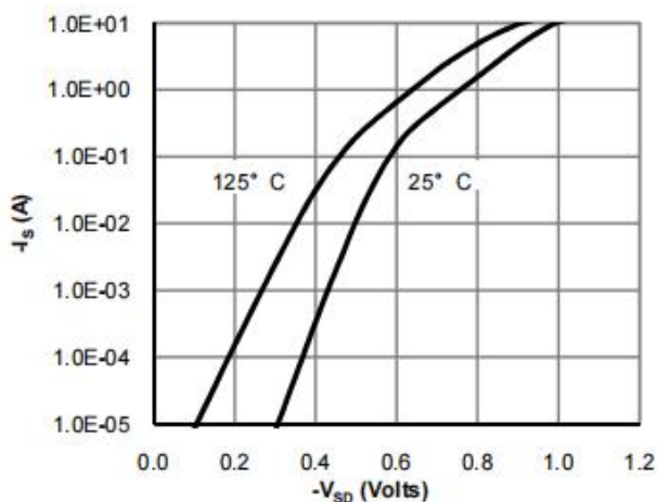
Figure 7: Diode Characteristics
