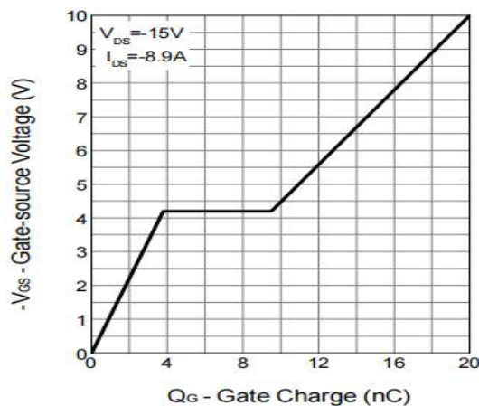
Figure 6: Gate-Charge Characteristics
