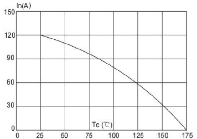
Figure 8: Drain Current vs. Tc
