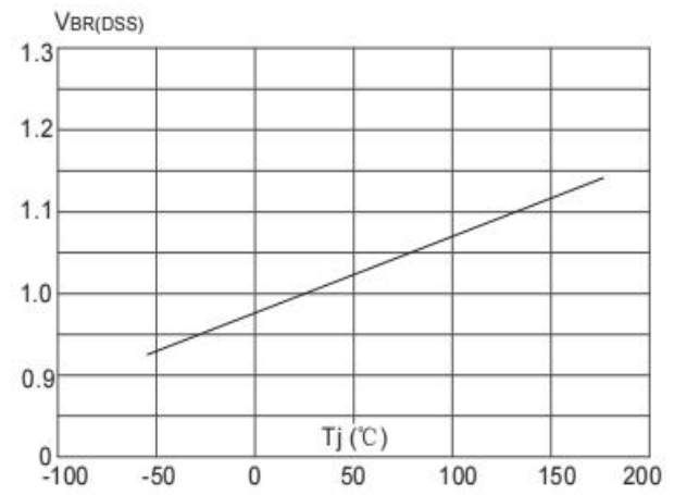
Figure 4: Breakdown Voltage vs. T_J
