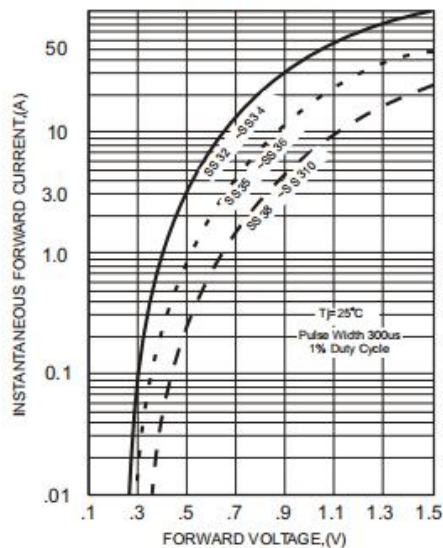
FIG.2-TYPICAL FORWARD CHARACTERISTICS
