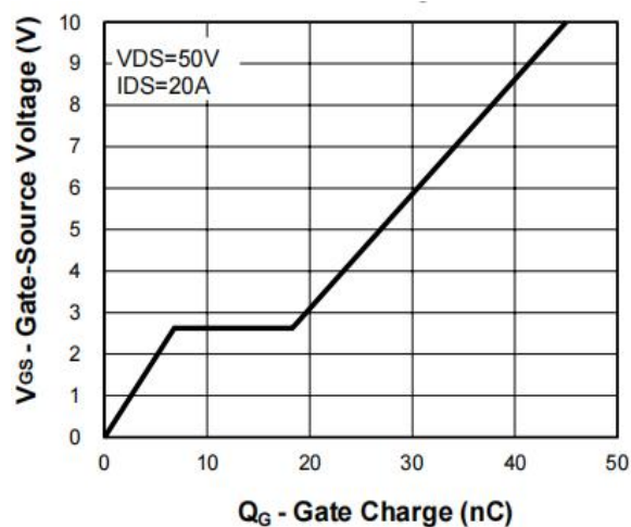
Figure 6: Gate-Charge Characteristics
