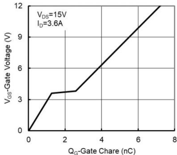
Figure 6: Gate-Charge Characteristics
