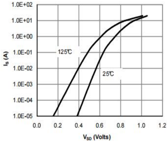
Figure 9: Diode Characteristics
