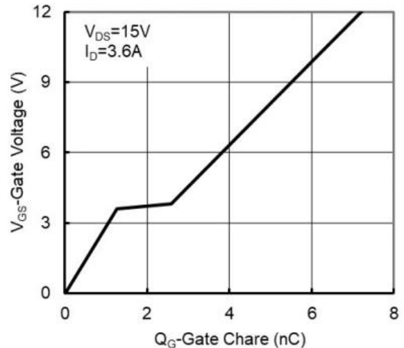
Figure 6: Gate-Charge Characteristics
