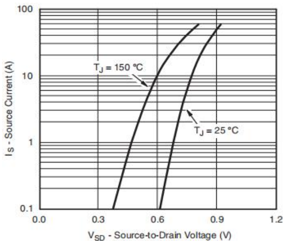
Figure 3: Diode Characteristics
