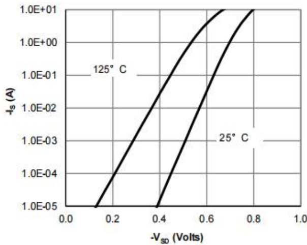
Figure 3: Diode Characteristics
