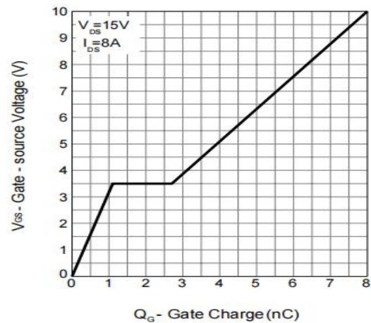
Figure 6: Gate-Charge Characteristics
