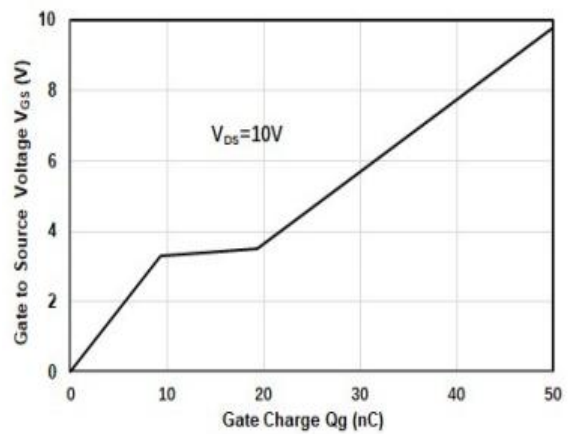
Figure 6: Gate-Charge Characteristics
