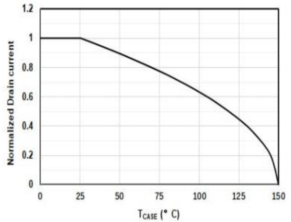
Figure 4: Drain Current vs. Temperature
