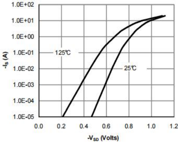
Figure 7: Diode Characteristics
