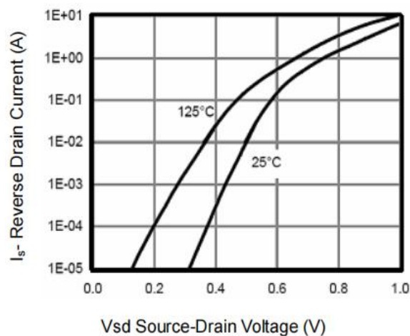
Figure 9: Diode Characteristics
