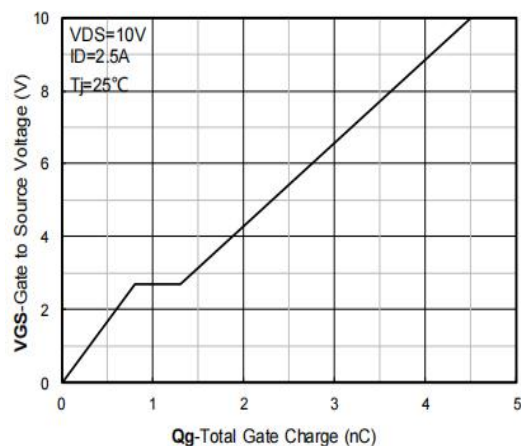
Figure 6: Gate-Charge Characteristics
