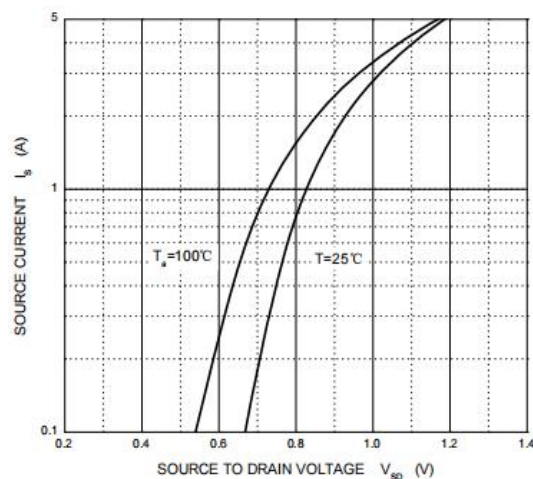
Figure 6: Diode Characteristics
