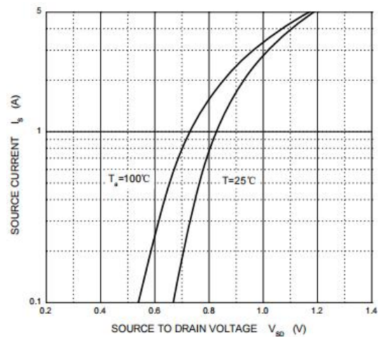
Figure 6: Diode Characteristics
