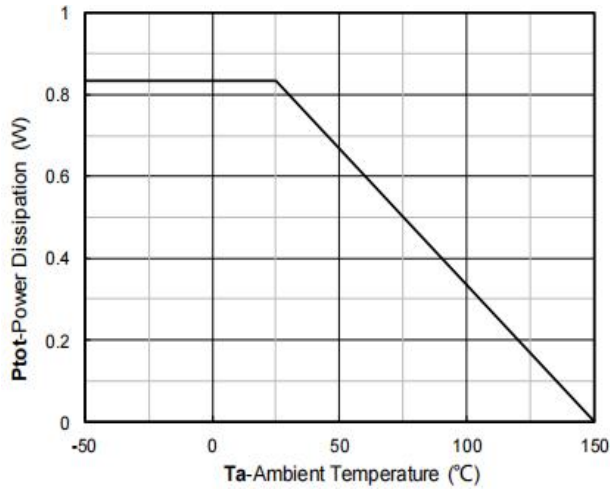
Figure 7: Power Dissipation vs. Temperature
