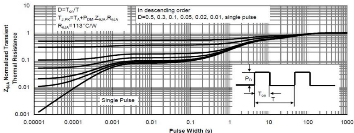
Figure 10: Transient Thermal Response Curve
