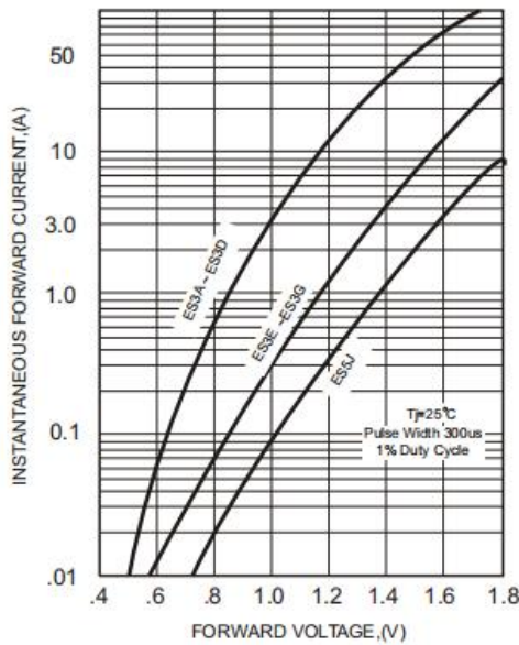
FIG.3-TYPICAL FORWARD CHARACTERISTICS
