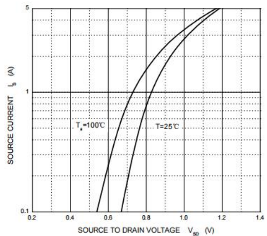
Figure 6: Diode Characteristics
