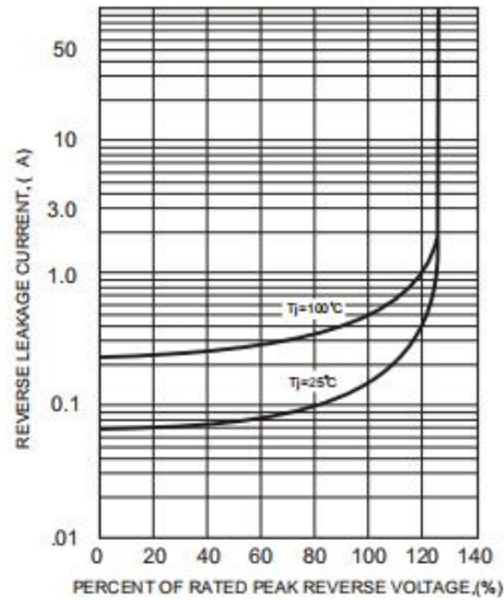
FIG.4-TYPICAL REVERSE CHARACTERISTICS
