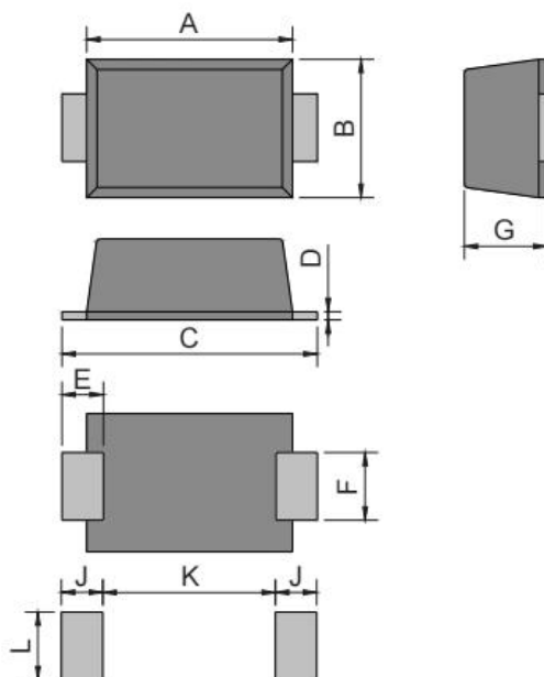
SOD-123FL
