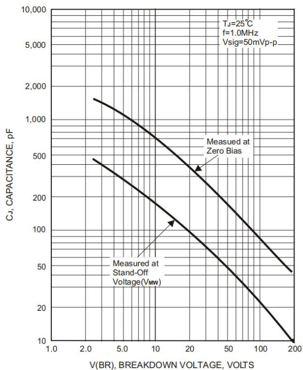
FIG.4-TYPICAL JUNCTION CAPACITANCE
