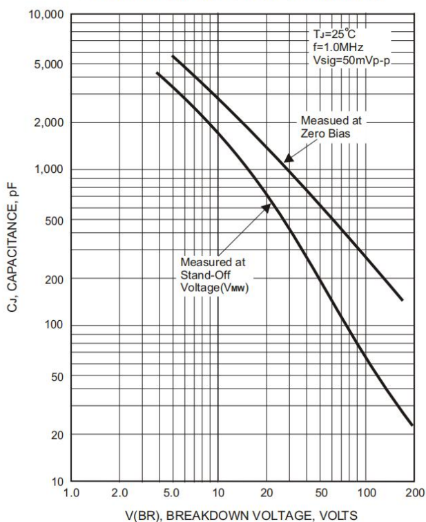
FIG.4-TYPICAL JUNCTION CAPACITANCE
