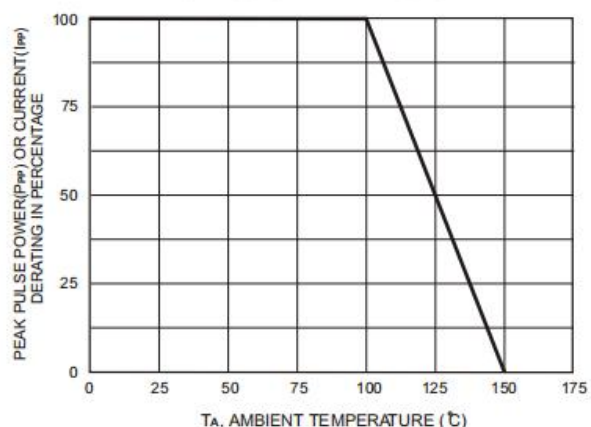
FIG.2-PULSE DERATING CURVE
