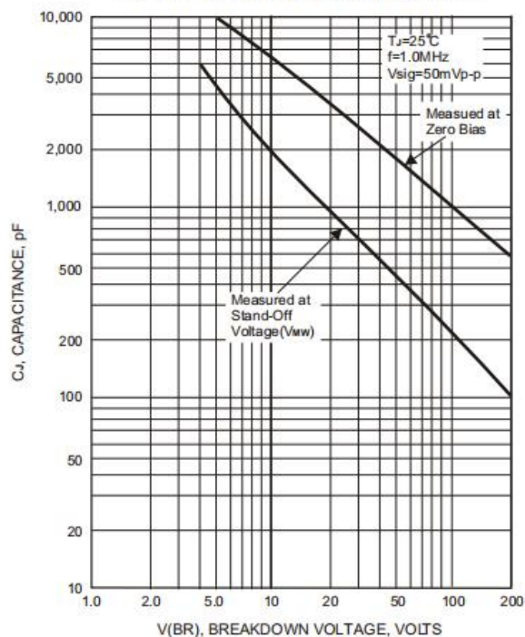
FIG.4-TYPICAL JUNCTION CAPACITANCE
