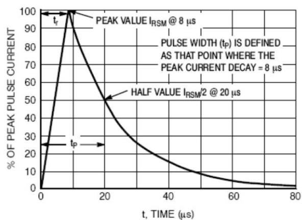
Figure 1. 8 x 20 μs Pulse Waveform
