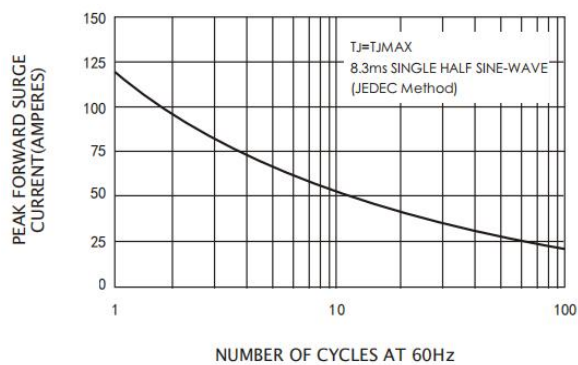
Figure 2: Forward Surge Current Curve
