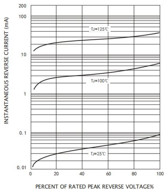
Figure 4: Reverse Characteristics
