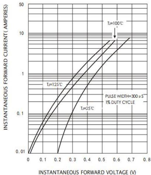
Figure 3: Forward Characteristics
