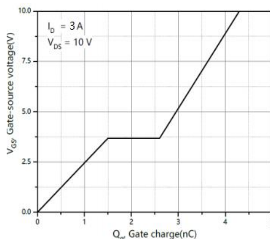
Figure 6: Gate-Charge Characteristics
