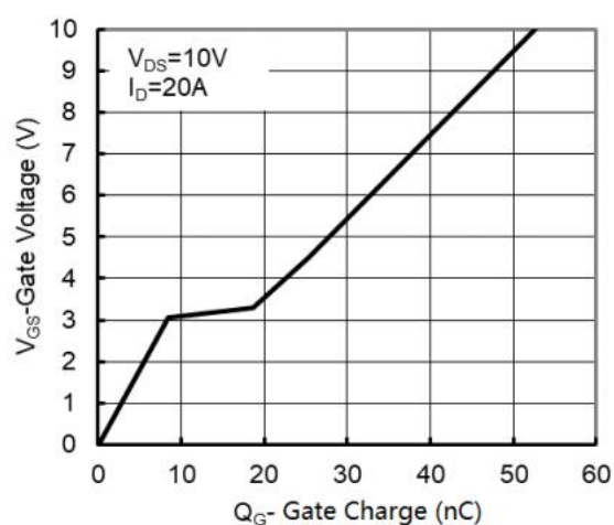
Figure 6: Gate-Charge Characteristics
