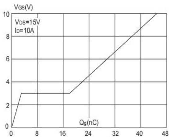
Figure 6: Gate-Charge Characteristics
