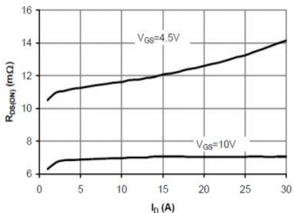
Figure 3: On-Resistance vs. ID
