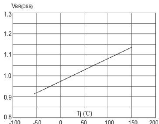
Figure 8: Breakdown Voltage vs. T_J
