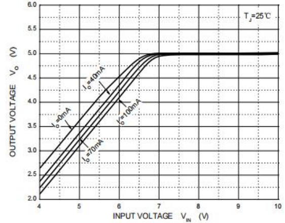
Figure 2: Dropout Characteristics
