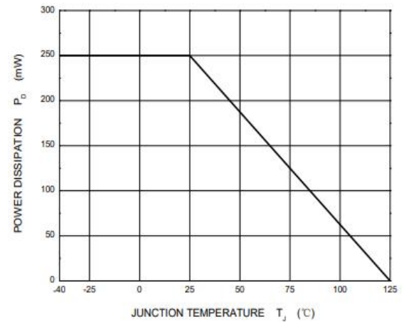
Figure 6: Power Characteristics
