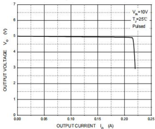
Figure 4: Output Characteristics
