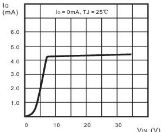
Figure 3: Quiescent Current Characteristics
