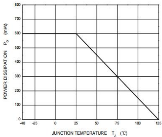
Figure 6: Power Characteristics
