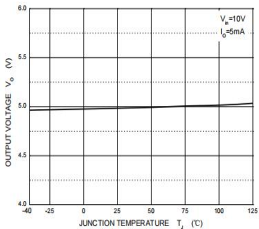
Figure 5: Temperature Characteristics
