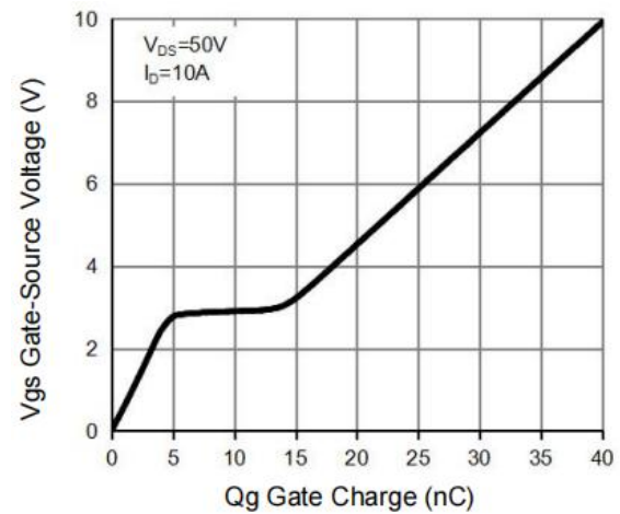
Figure 6: Gate-Charge Characteristics
