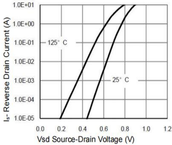
Figure 7: Diode Characteristics
