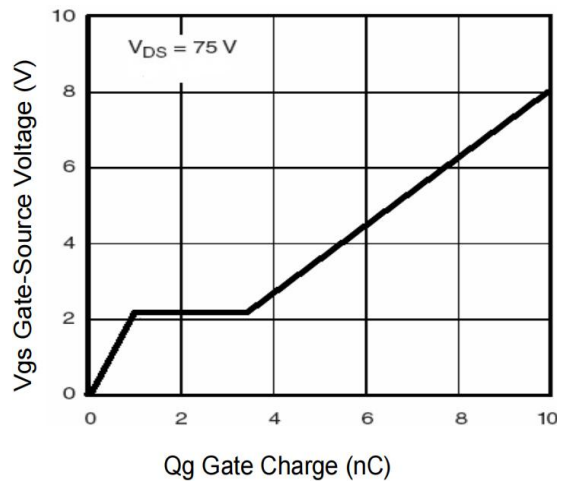
Figure 6: Gate-Charge Characteristics
