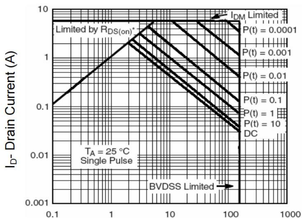
Vds Drain-Source Voltage (V) Figure 8: Safe Operating Area
