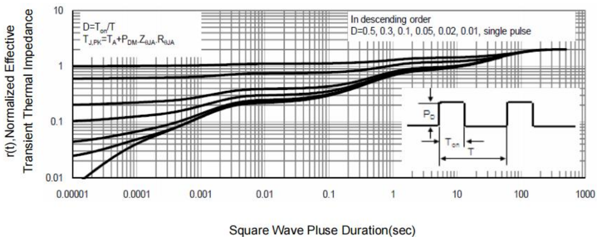
Square Wave Pluse Duration(sec) Figure 9: Transient Thermal Response Curve
