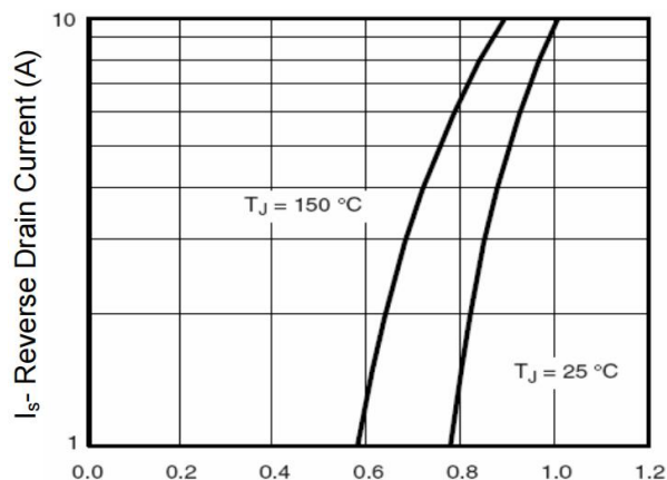
Vsd Source-Drain Voltage (V) Figure 7: Diode Characteristics
