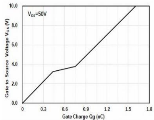
Figure 6: Gate-Charge Characteristics
