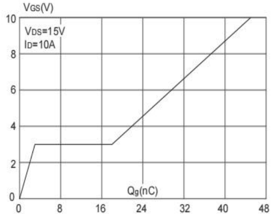
Figure 6: Gate-Charge Characteristics
