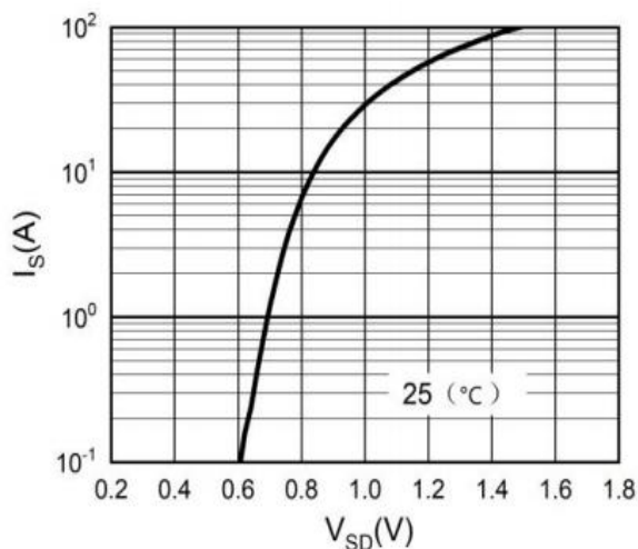
Figure 7: Diode Characteristics
