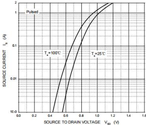
Figure 5: Diode Characteristics
