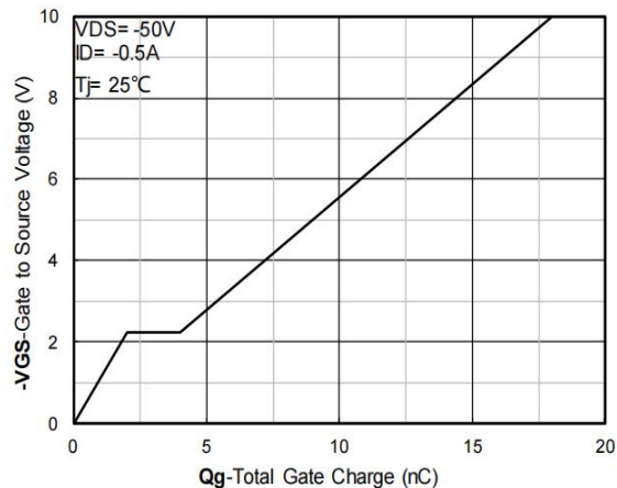
Figure 6: Gate-Charge Characteristics
