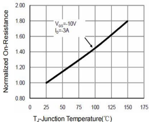
Figure 4: On-Resistance vs.
