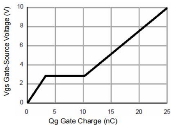
Figure 6: Gate-Charge Characteristics
