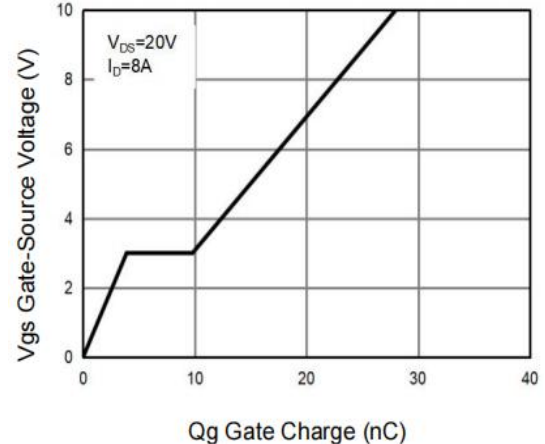
Figure 6: Gate-Charge Characteristics
