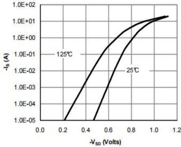
Figure 7: Diode Characteristics
