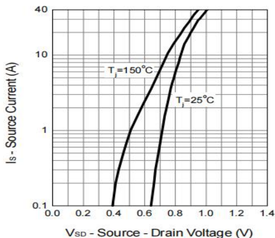
Figure 9: Diode Characteristics
