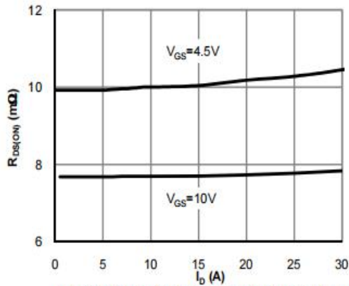
Figure 3: On-Resistance vs. Drain Current and Gate
