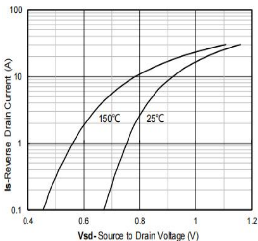
Figure 7: Diode Characteristics
