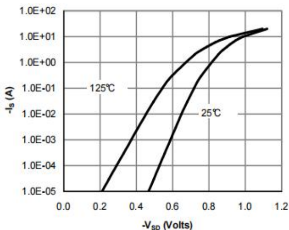
Figure 7: Diode Characteristics
